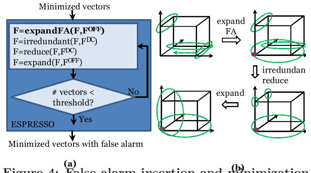
Figure 4: False alarm insertion and minimization
