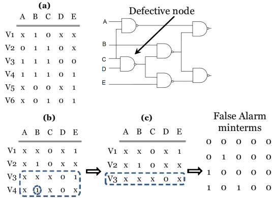
Figure 3: Example of failing C17 circuit; (a) faulty cubes before minimization; (b) faulty cubes after minimization; (c) cubes after adding false alarms
