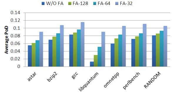
Figure 6: Probability of Detection for a single fault
