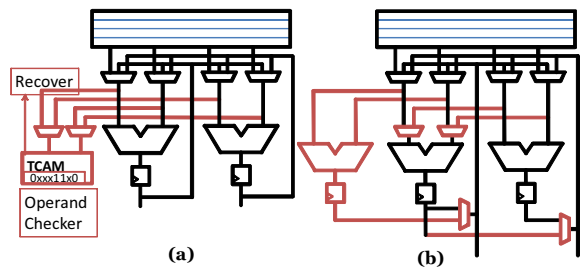
Figure 2: Protect a 2-issue faulty processor using (a) a checker unit; (b) a redundant module
