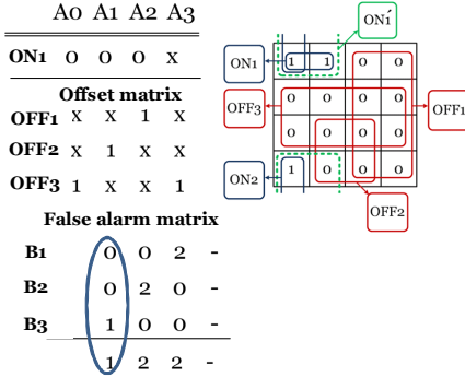
Figure 5: False alarm insertion for one cube
